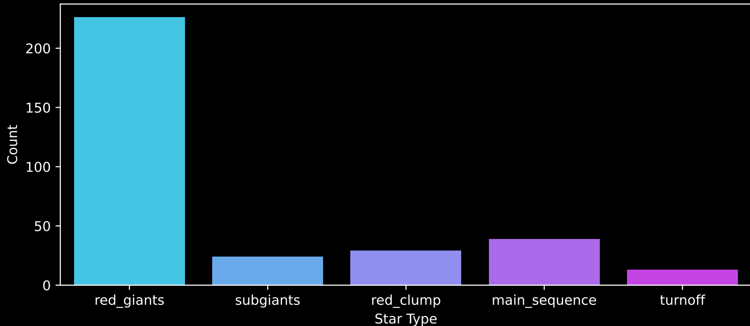
APOGEE DR17 Field: [173+00] Count plot of Star Type
