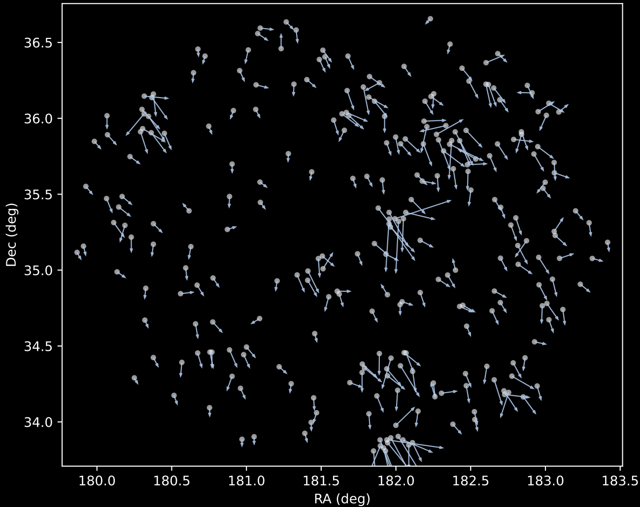
APOGEE DR17 Cluster 1 Proper Motion Vectors (n=265)
