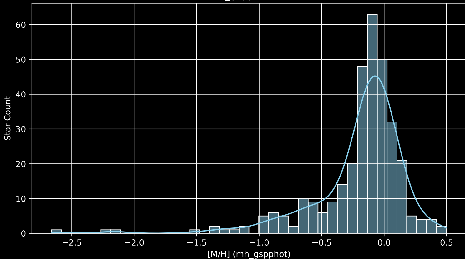
APOGEE DR17 Field: [173+00 [M/H] (mh_gspphot) (n= 325)
