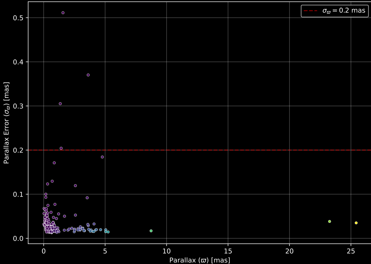
APOGEE DR17 Field: [173+00] Parallax Quality (n= 331)
