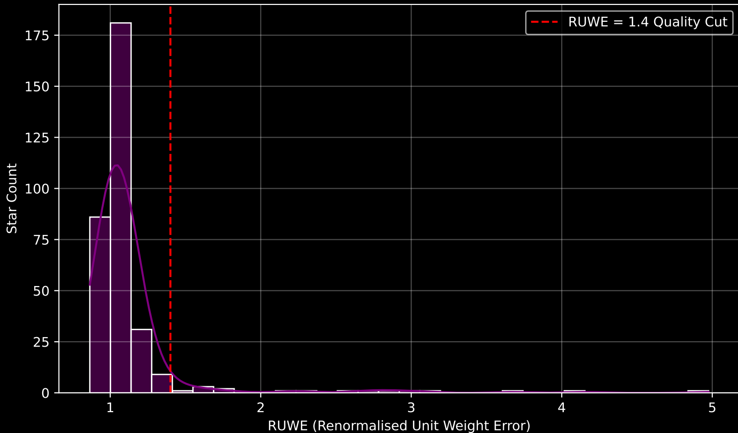
GAPOGEE DR17 Field [173+00] RUWE Distribution (n= 323)
