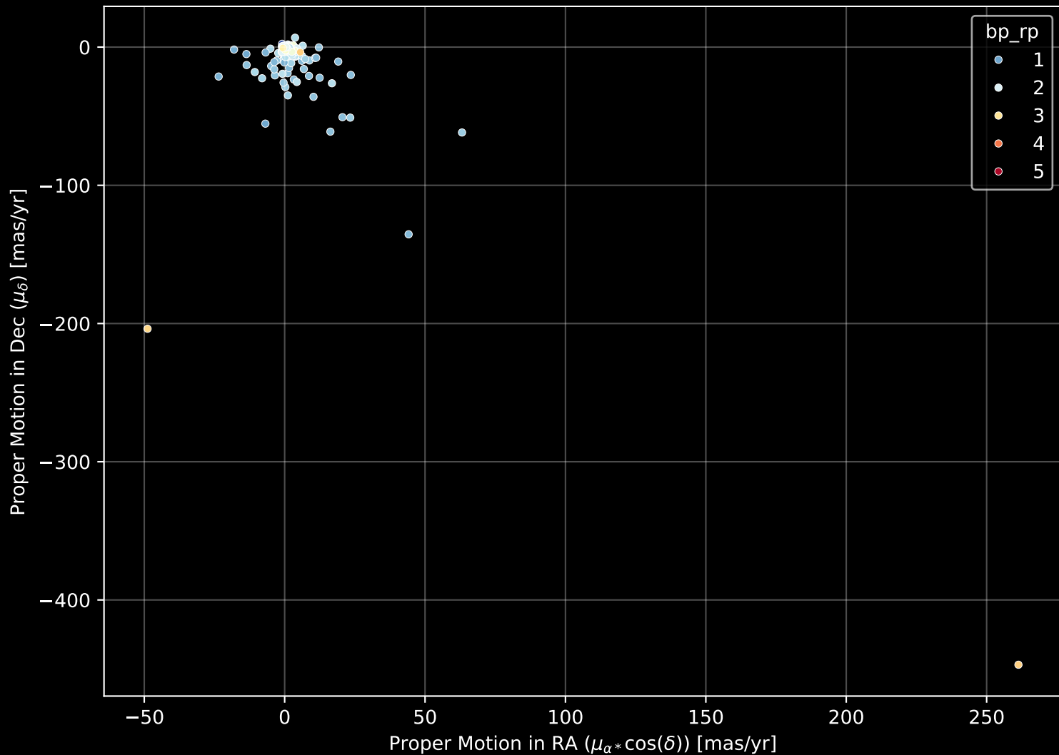
APOGEE DR17 Field: [173+00] Proper Motion Diagram (n= 331)
